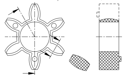
picture 17.2: ROTEX® spider
