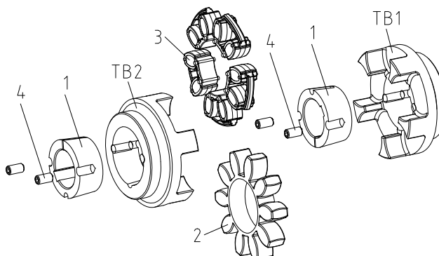
picture 8: ROTEX® design with taper clamping sleeve
