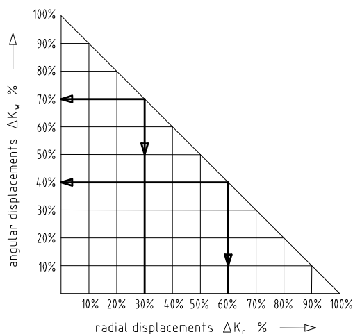
picture 15: combinations of displacement
