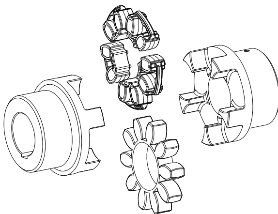
picture 16: ROTEX® coupling
